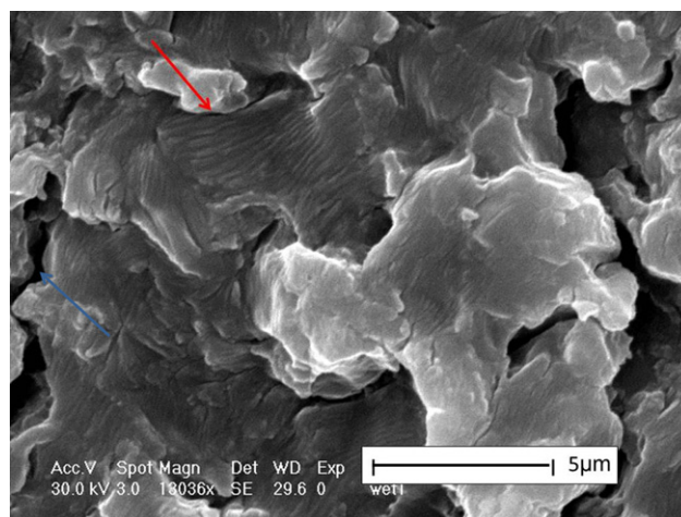
Figure 6 Fatigue striation (red arrow) between transgranular fractures (blue arrow) indicating fatigue fracture. Taken from a 3.75-mm implant, with maximum load of 810 N and 73,983 cycles to failure. Note that fatigue striations are only discernable at relatively large magnifications, on the order of \times 10\text{k} .
