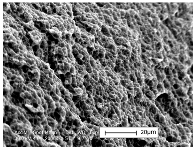
Figure 7 A view of final fracture (monotonic overload). Found on the fracture surface of the implant described at Figure 14. Final fracture failure is characterized by equiaxed dimples.
