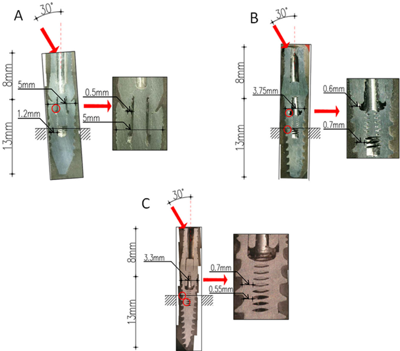
Figure 3 Metallographic section of the three-implant diameter testing group. A: 5-mm implant. B: 3.75-mm implant. C: 3.3-mm implant. The length and width of the implant and abutment are indicated. The upper red arrow indicates testing force applied to the implant abutment and the force direction at an angle of 30° off-axis. The red circles indicate the different fracture modes found at each implant diameter. The magnified picture shows the fracture location and the corresponding metal width at the fracture location.
