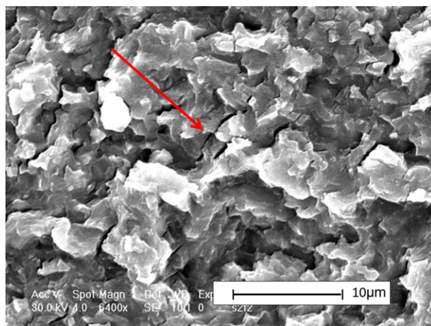
Figure 5 A view of a fatigue fracture mode found in the fracture surface of a 3.3-mm implant. The maximum load was 438 N and the specimen failed after 1,420,000 cycles. Fatigue failure is characterized by transgranular fracture with many secondary parallel cracks (arrow) perpendicular to the local crack-front propagation.
